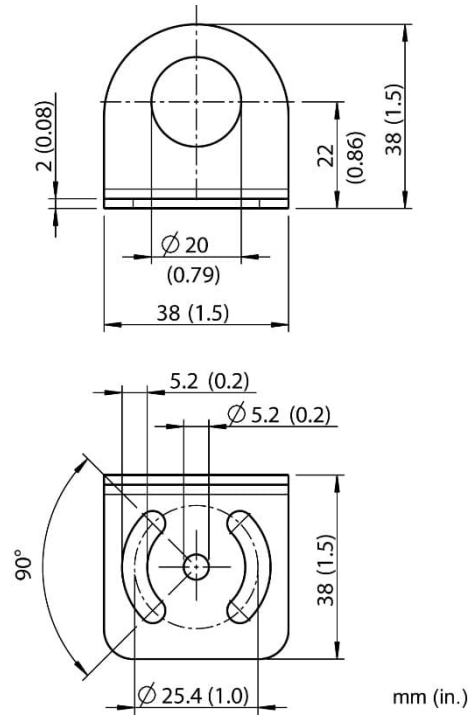
Figure 70: Dimensions of Fixed Mounting Bracket (XXXMI3100FB)
