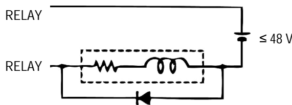
Figure 24: Spike Voltage Limitation for the Alarm Relay
